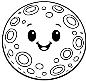
Mercury
